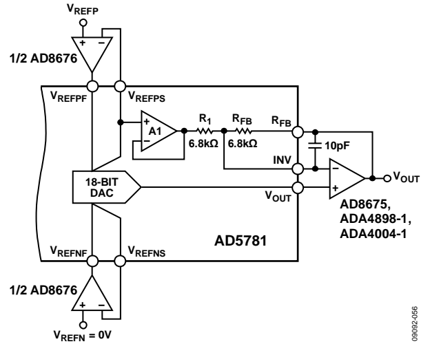
Figure 52. Output Amplifier in Gain of Two Configuration
