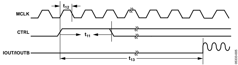
Figure 5. CTRL Timing
