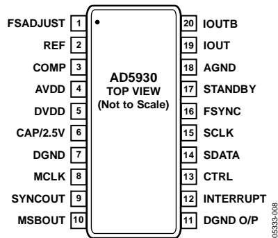
Figure 8. Pin Configuration
