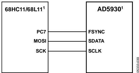
Figure 37. 68HC11/68L11 to AD5930 Interface
