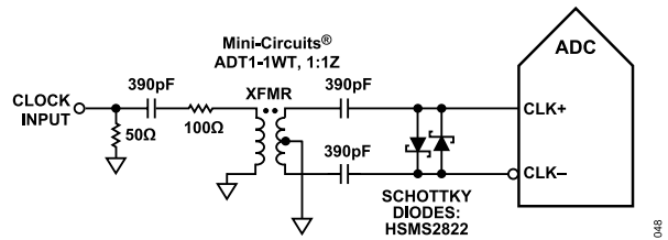
Figure 32. Transformer-Coupled Differential Clock (Up to 200 MHz)
