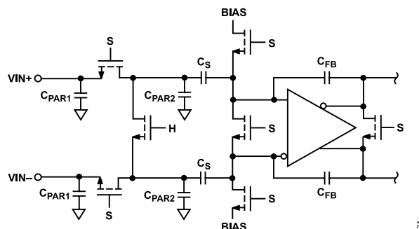
Figure 26. Switched-Capacitor Input
