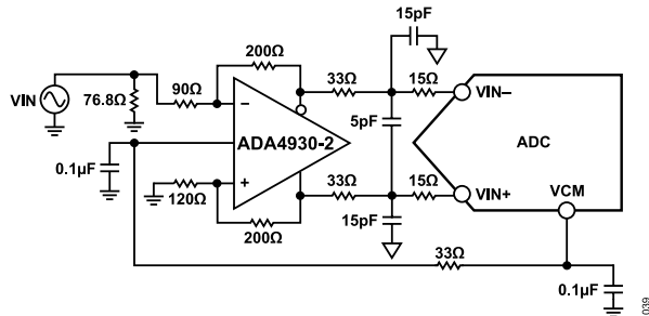
Figure 27. Differential Input Configuration Using the ADA4930-2
