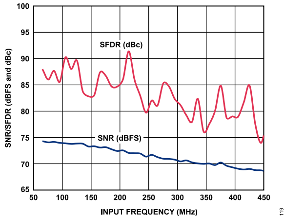
Figure 12. AD6649 Single-Tone SNR/SFDR vs. Input Frequency ( f_{IN} )
