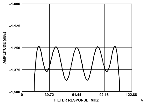
Figure 42. Low Latency FIR Filter Pass-Band Response at 245.76 MSPS (Fixed-Frequency NCO, 95 MHz FIR Filter Mode)
