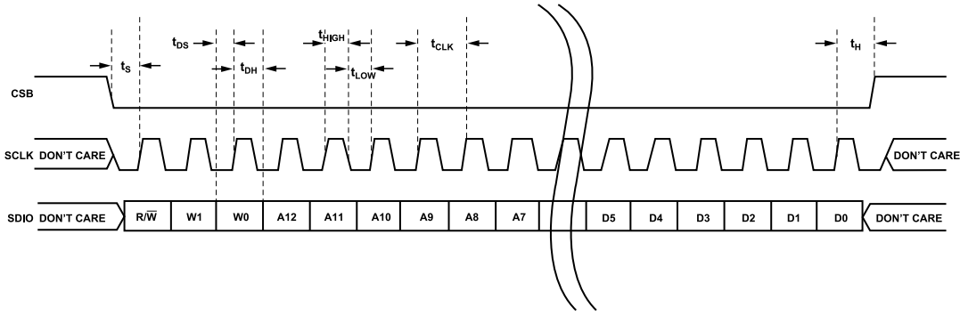
Figure 46. Serial Port Interface Timing Diagram
