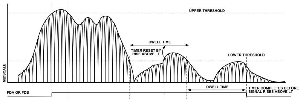
Figure 45. Threshold Settings for FDA and FDB Signals
