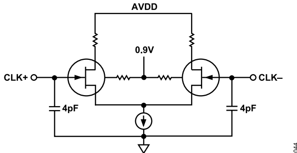
Figure 31. Simplified Equivalent Clock Input Circuit
