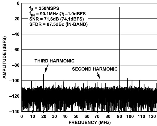
Figure 6. AD6649 Single-Tone FFT with f_{IN} = 90.1 MHz
