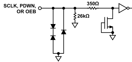
Figure 23. Equivalent SCLK, PDWN, or OEB Input Circuit
