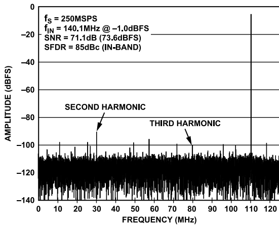
Figure 7. AD6649 Single-Tone FFT with f_{IN} = 140.1 MHz
