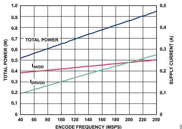
Figure 37. AD6649 Power and Current vs. Sample Rate
