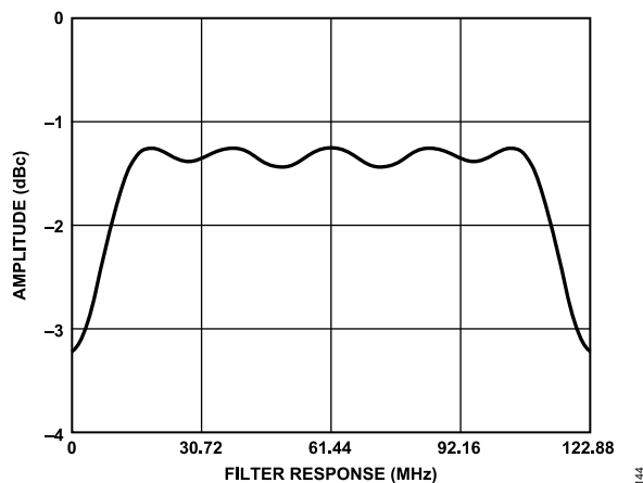
Figure 41. Low Latency FIR Filter Composite Response at 245.76 MSPS (Fixed-Frequency NCO, 95 MHz FIR Filter Mode)
