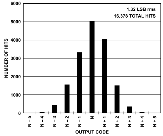
Figure 18. AD6649 Grounded Input Histogram
