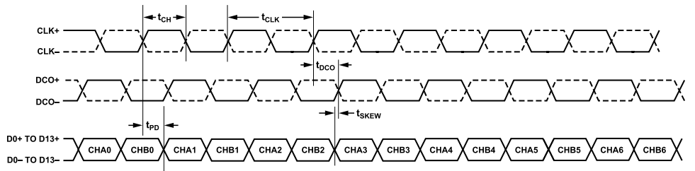
Figure 2. Interleaved LVDS Mode Data Output Timing
