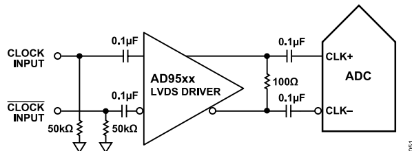
Figure 35. Differential LVDS Sample Clock (Up to 625 MHz)
