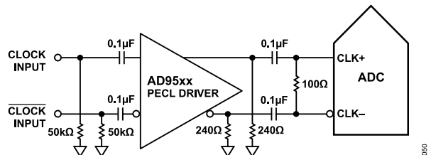
Figure 34. Differential PECL Sample Clock (Up to 625 MHz)
