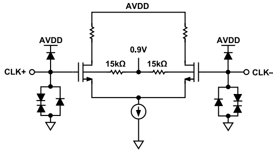
Figure 20. Equivalent Clock Input Circuit
