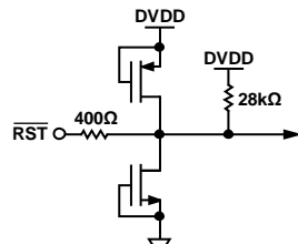
Figure 26. \overline{RST} Equivalent Circuit
