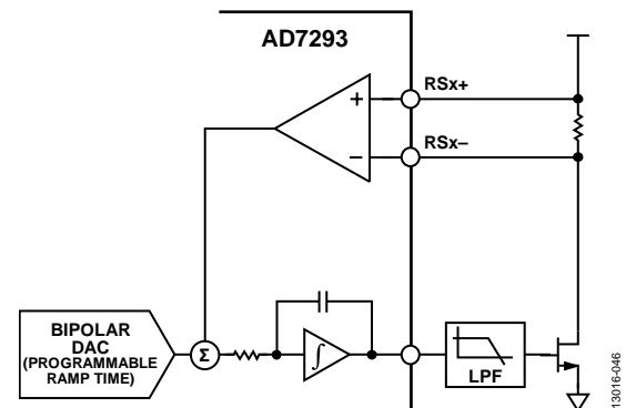
Figure 46. Closed-Loop Control
