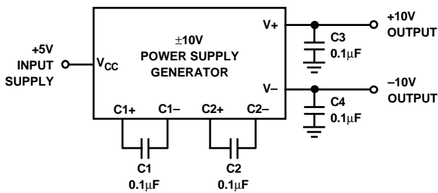
Figure 7. Charge Pump Voltage Generator
