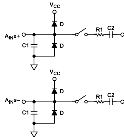
Figure 28. Equivalent Analog Input Circuit, Conversion Phase—Switches Open, Track Phase—Switches Closed
