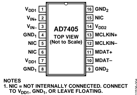
Figure 4. Pin Configuration
