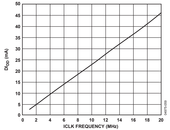
Figure 38. Decimate \times 32 , D_{IDD} vs. ICLK Frequency ( V_{DD} = 2.5\text{ V} )
