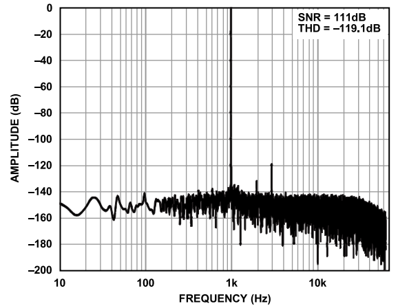
Figure 14. FFT, Median Mode, Sinc5 Filter, -0.25 dBFS
