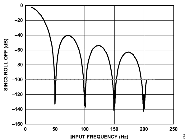
Figure 72. Sinc3 Filter Frequency Response Showing 50 Hz Rejection, 50 Hz ODR, \times 163,840 Decimation
