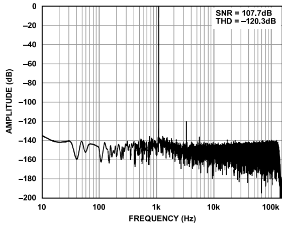
Figure 10. FFT, Fast Mode, Low Ripple FIR Filter, -0.25 dBFS
