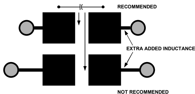
Figure 33. Recommended Pad Outline for Bypass Capacitors
