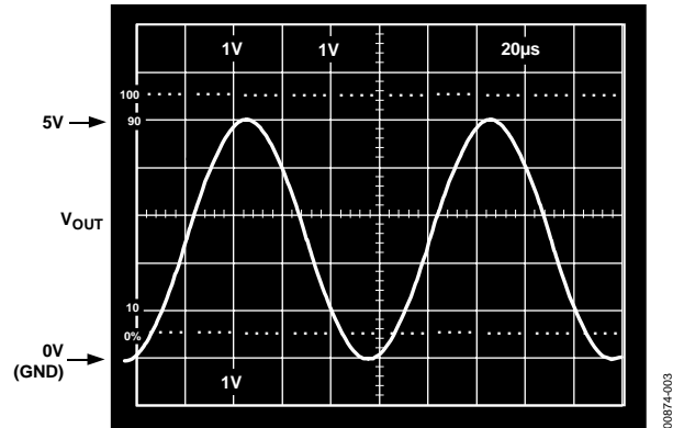
Figure 3. Gain of 2 Amplifier; V_S = 5V, 0V , V_{IN} = 2.5V Sine Centered at 1.25V , R_L = 100\Omega
