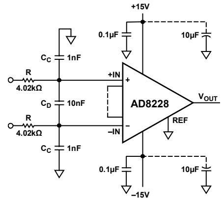
Figure 47. RFI Suppression
