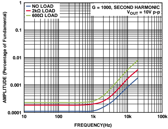
Figure 53. Second Harmonic Distortion vs. Frequency, G = 1000
