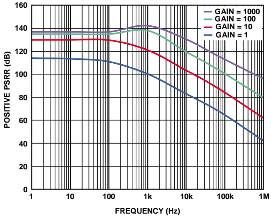
Figure 18. Positive PSRR vs. Frequency
