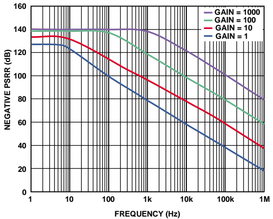
Figure 19. Negative PSRR vs. Frequency
