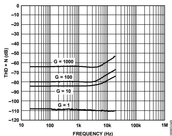
Figure 49. Total Harmonic Distortion vs. Frequency, 10 Hz to 22 kHz Band-Pass Filter, 2\text{ k}\Omega Load
