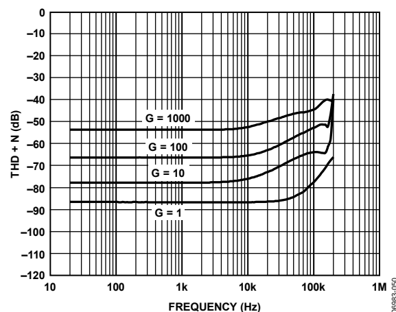
Figure 50. Total Harmonic Distortion vs. Frequency, 10 Hz to 500 kHz Band-Pass Filter, 2\text{ k}\Omega Load
