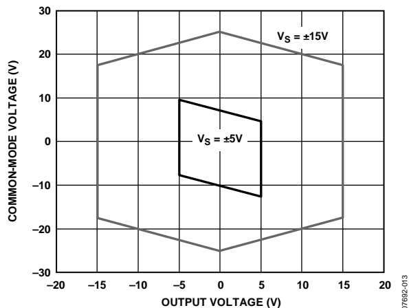
Figure 15. Input Common-Mode Voltage vs. Output Voltage, ±15 V and ±5 V Supplies
