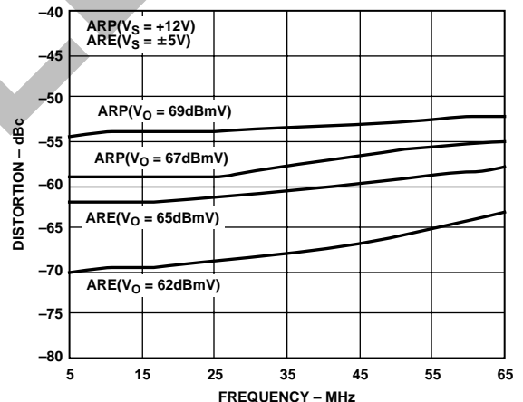
Figure 1. Worst Harmonic Distortion vs. Frequency
