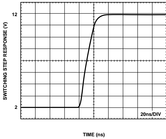
Figure 13. Invert Switching Step Response (Rising Edge), 10 V Step, C_L = 200 pF
