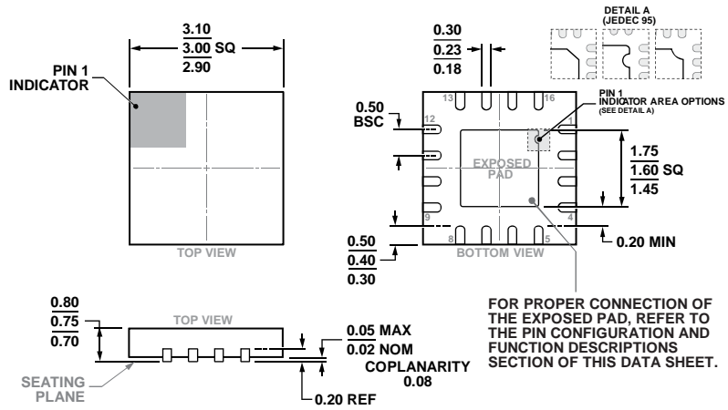
Figure 57. 16-Lead Lead Frame Chip Scale Package [LFCSP] 3 mm x 3 mm Body and 0.75 mm Package Height (CP-16-22)
