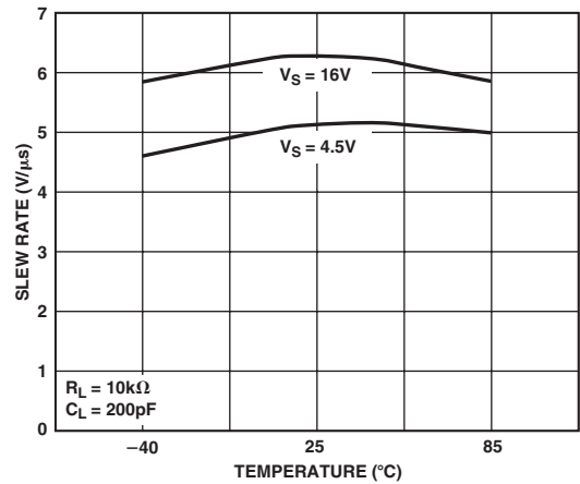
TPC 11. Slew Rate vs. Temperature
