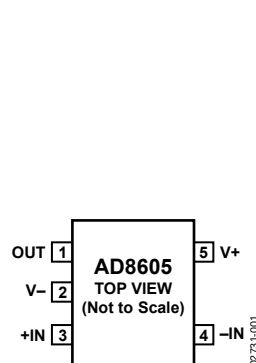
Figure 1. 5-Lead SOT-23 (RJ Suffix)
