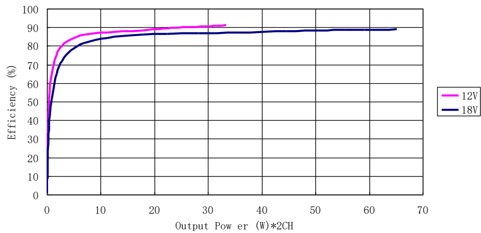
Efficiency (Stereo 6Ω load) / 2ch
