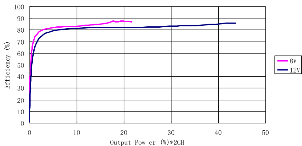
Efficiency (Stereo 4Ω load) / 2ch
