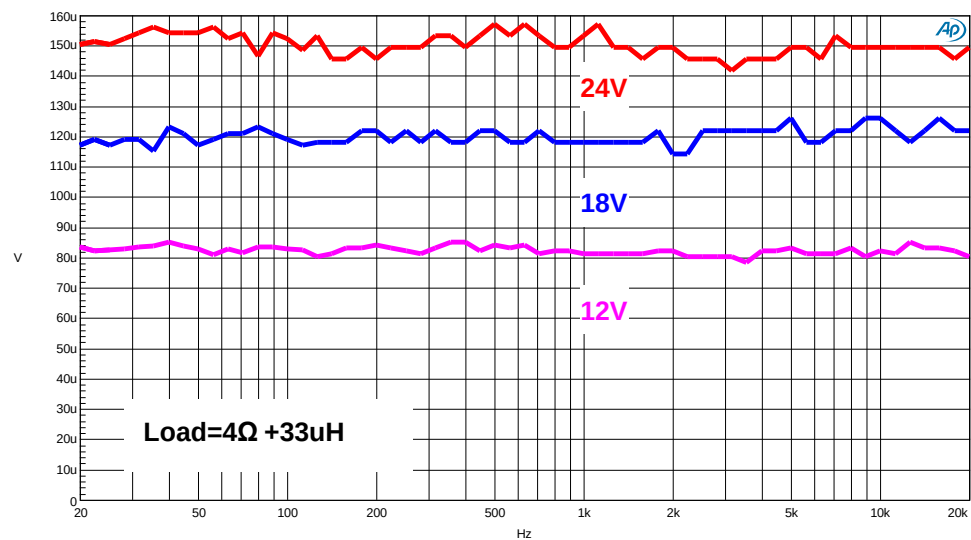
Noise (Mono 4Ω load)
