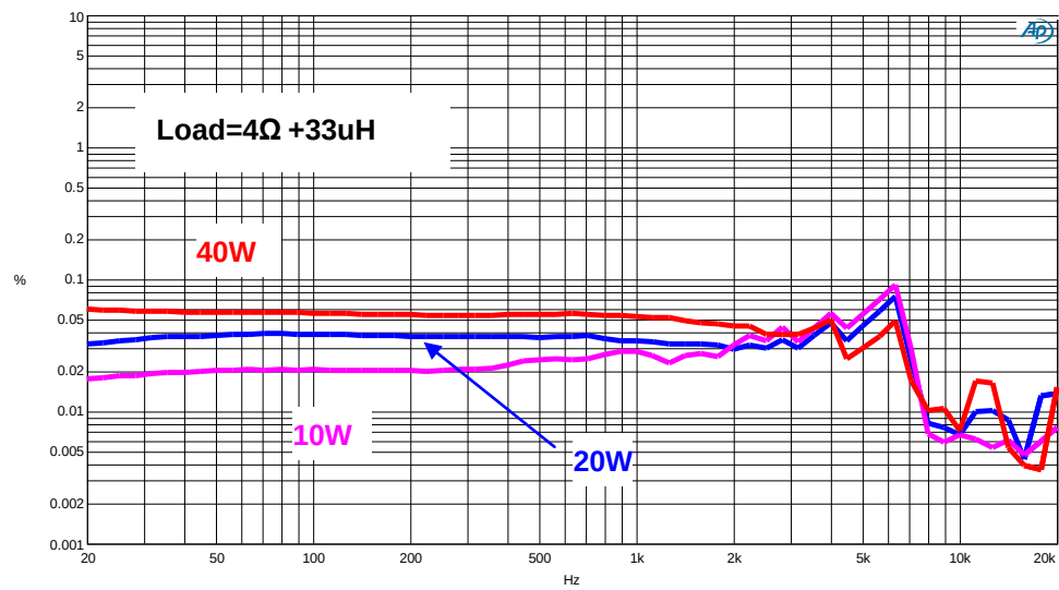
THD + N (%) v.s. Frequency (24V Mono 4Ω load)
