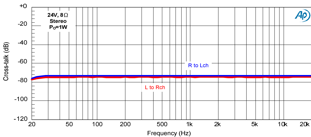
Cross-talk (Stereo, BTL)
