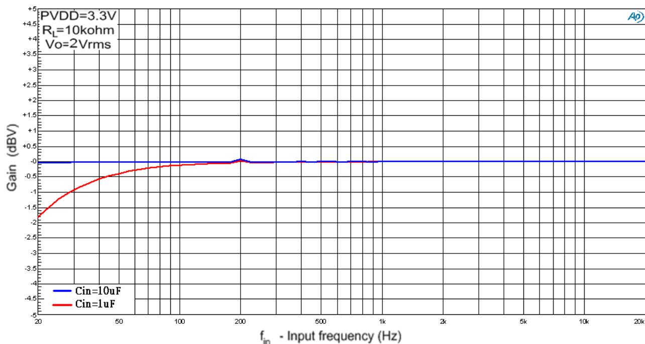
Gain vs. Signal Frequency
