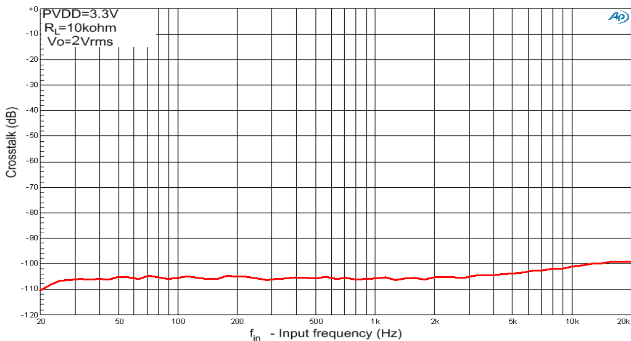
Cross-talk vs. Signal Frequency
