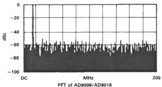
400MSPS: F_{IN} = 14.8\text{MHz} ; V_{IN} = 1.0\text{dB Below FS}
