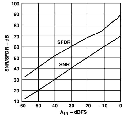
TPC 9. SNR/SFDR vs. A_{\text{IN}} (Input Amplitude) ( f_{\text{IN}} = 500 \text{ kHz} , Input Span = 2 V p-p, V_{\text{CM}} = 2.5 \text{ V} )
