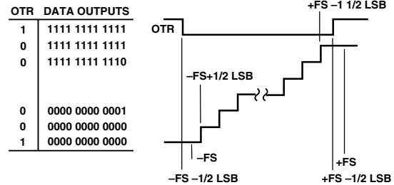
Figure 27. Output Data Format
