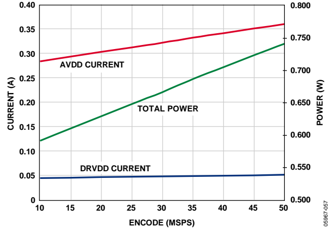
Figure 69. Supply Current vs. f_{SAMPLE} for f_{IN} = 10.3 \text{ MHz} , AD9222- 50
