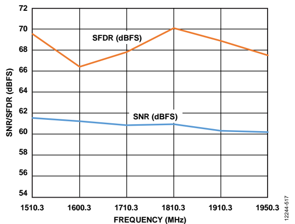
Figure 40. SNR/SFDR vs. Input Frequency ( f_{IN} ); 1500 MHz < f_{IN} < 2000 MHz; Buffer Current = 8.5\times (Uses Circuit Shown in Figure 64)
