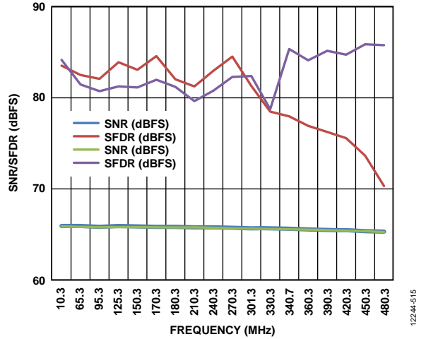
Figure 38. SNR/SFDR vs. Input Frequency ( f_{IN} ); f_{IN} < 500 MHz; Buffer Current = 2.5\times and 4.5\times (Uses Circuit Shown in Figure 63)
