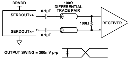
Figure 94. AC-Coupled Digital Output Termination Example
