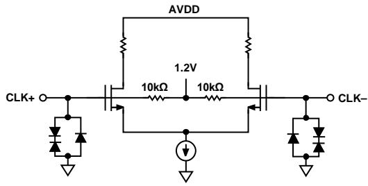
Figure 35. CLK± Inputs
