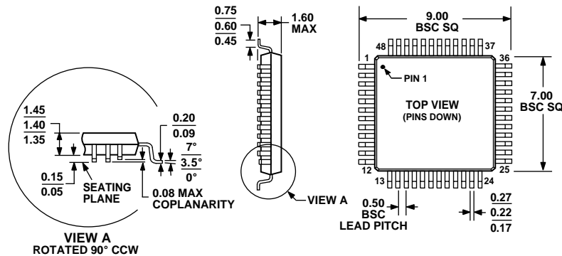
COMPLIANT TO JEDEC STANDARDS MS-026-BBC Figure 74. 48-Lead Low Profile Quad Flat Package [LQFP] (ST-48) Dimensions shown in millimeters
