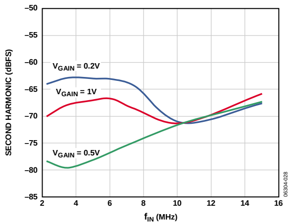
Figure 32. Second-Order Harmonic Distortion vs. Frequency, A_{IN} = -0.5\text{ dBFS}
