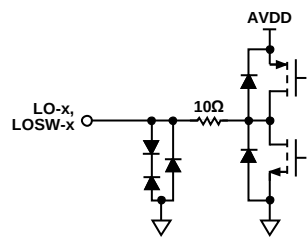
Figure 6. Equivalent LNA Output Circuit
