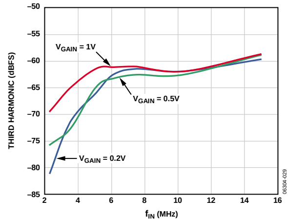
Figure 33. Third-Order Harmonic Distortion vs. Frequency, A_{IN} = -0.5\text{ dBFS}
