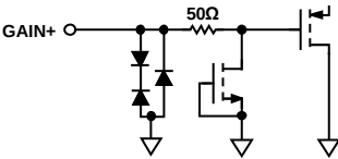
Figure 15. Equivalent GAIN+ Input Circuit
