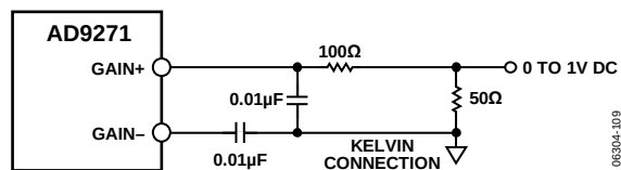
Figure 51. Single-Ended GAIN± Pins Configuration
