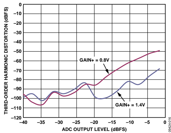
Figure 17. Third-Order Harmonic Distortion vs. ADC Output Level, AOUT = -1.0 dBFS
