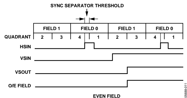
Figure 11. VSYNC Filter—Even
