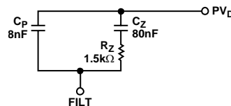
Figure 6. PLL Loop Filter Detail
