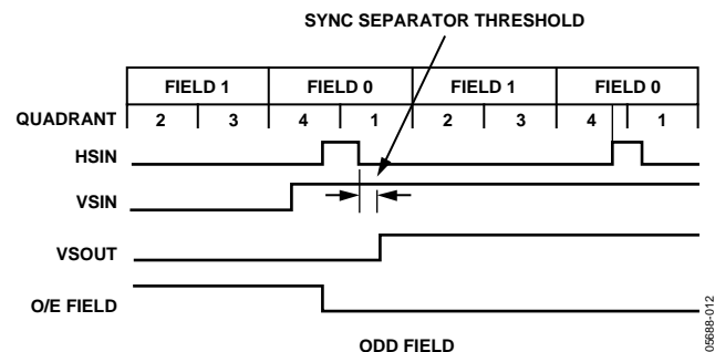
Figure 12. VSYNC Filter—Odd
