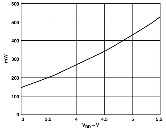
TPC 12. Output Power vs. V_{DD} , C_{LOAD} = 10\text{ pF}
