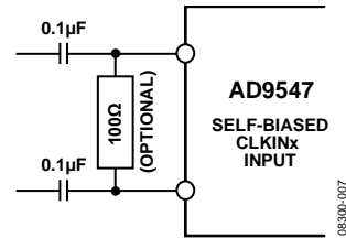
Figure 30. CLKINx Input
