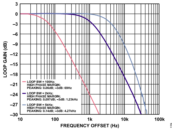
Figure 28. Closed-Loop Transfer Function for 100 Hz, 2 kHz, and 5 kHz Loop Bandwidth Settings; High Phase Margin Loop Filter Setting
