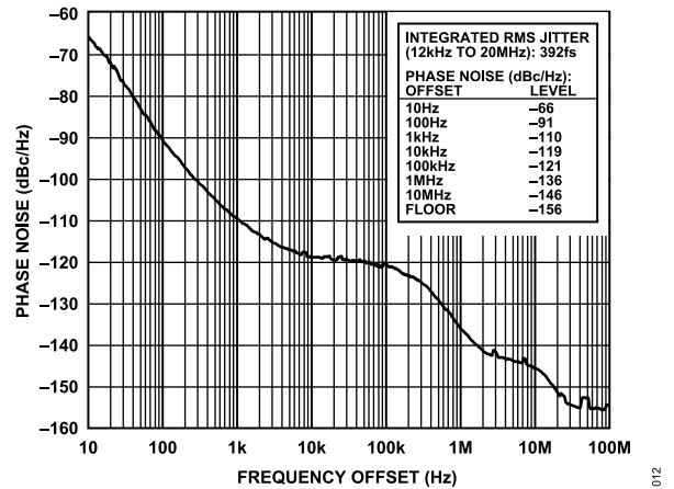
Figure 13. Absolute Phase Noise (Output Driver = HSTL), f_R = 19.44 MHz, f_{OUT} = 312.5 MHz, DPLL Loop BW = 0.1 Hz, f_{SYS} = 19.2 MHz TCXO
