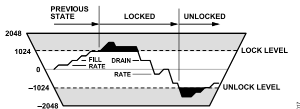
Figure 39. Lock Detector Diagram
