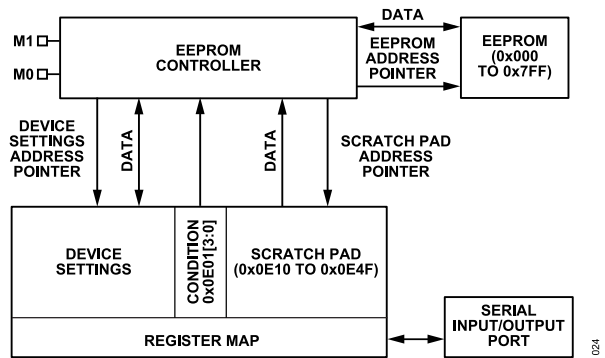
Figure 44. EEPROM Functional Diagram
