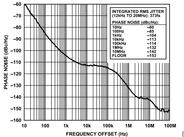
Figure 11. Absolute Phase Noise (Output Driver = HSTL), f_R = 19.44 MHz, f_{OUT} = 644.53 MHz, DPLL Loop BW = 10 Hz, f_{SYS} = 19.2 MHz TCXO
