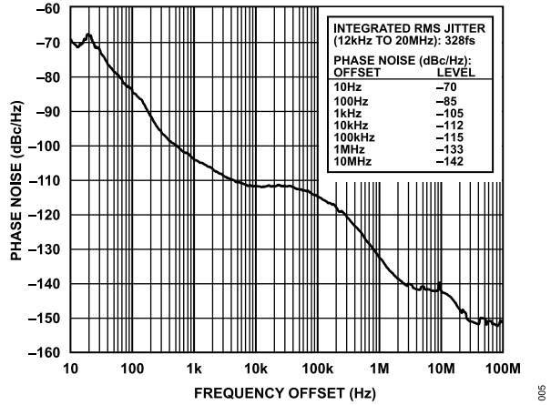
Figure 6. Absolute Phase Noise (Output Driver = HSTL), f_R = 19.44 MHz, f_{OUT} = 693.482991 MHz, DPLL Loop BW = 50 Hz, f_{SYS} = 49.152 MHz Crystal
