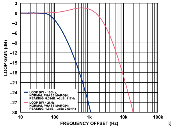
Figure 29. Closed-Loop Transfer Function for 100 Hz and 2 kHz Loop Bandwidth Settings; Normal Phase Margin Loop Filter Setting Note that bandwidth is defined as the point where the open loop gain = 0 dB.
