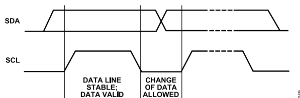
Figure 52. Valid Bit Transfer
