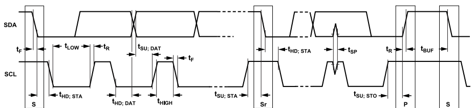
Figure 57. I 2 C Serial Port Timing
