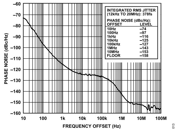
Figure 14. Absolute Phase Noise (Output Driver = 3.3 V CMOS), f_R = 19.44 MHz, f_{OUT} = 161.1328125 MHz, DPLL Loop BW = 10 Hz, f_{SYS} = 19.2 MHz TCXO
