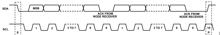
Figure 55. Data Transfer Process (Main Write Mode, 2-Byte Transfer)
