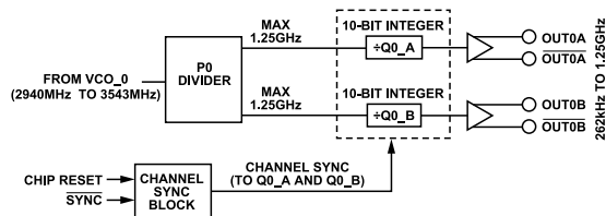
Figure 42. Clock Distribution Block Diagram from VCO_0
