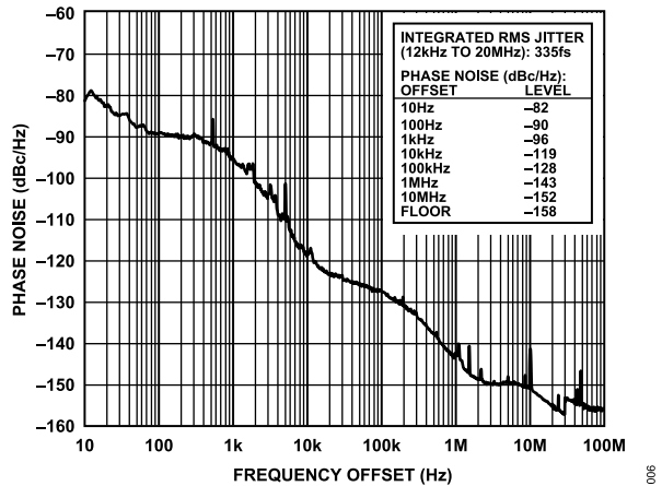
Figure 7. Absolute Phase Noise (Output Driver = HSTL), f_R = 19.44 MHz, f_{OUT} = 174.703 MHz, DPLL Loop BW = 1 kHz, f_{SYS} = 49.152 MHz Crystal
