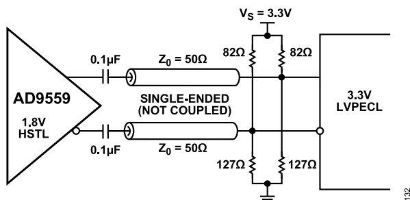
Figure 32. Interfacing the HSTL Driver to a 3.3 V LVPECL Input (This method incorporates impedance matching and dc-biasing for bipolar LVPECL
