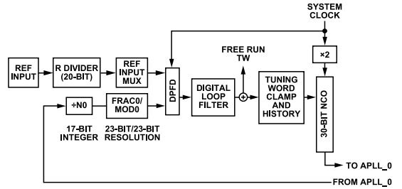
Figure 36. DPLL_0 Core
