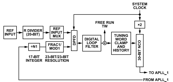
Figure 37. DPLL_1 Core
