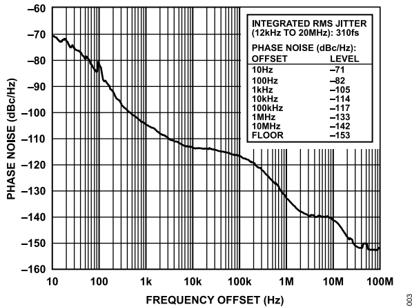
Figure 4. Absolute Phase Noise (Output Driver = HSTL), f_R = 19.44 MHz, f_{OUT} = 622.08 MHz, DPLL Loop BW = 50 Hz, f_{SYS} = 49.152 MHz Crystal
