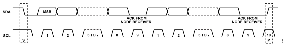
Figure 54. Acknowledge Bit
