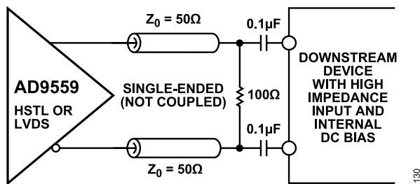
Figure 30. AC-Coupled LVDS or HSTL Output Driver (100 Ω resistor can be placed on either side of decoupling capacitors and should be as close to the destination receiver as possible.)
