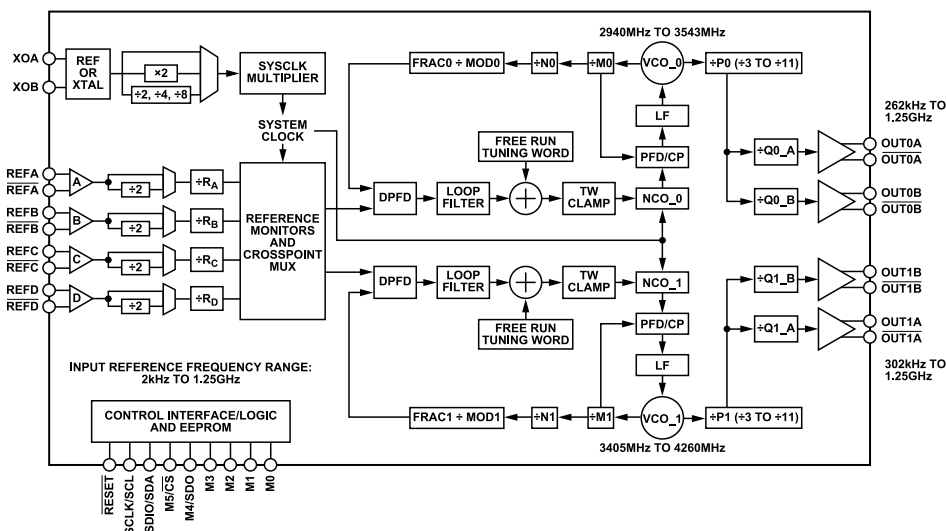
Figure 35. Detailed Block Diagram
