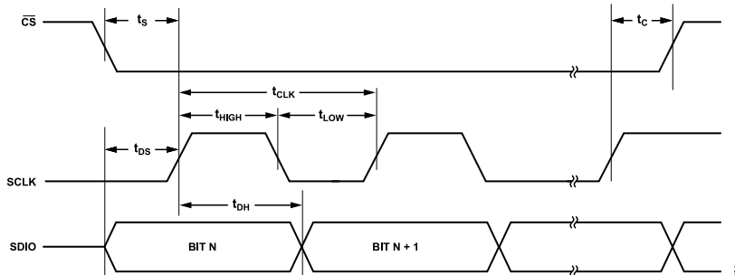
Figure 51. Serial Control Port Timing—Write
