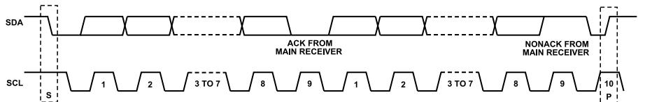
Figure 56. Data Transfer Process (Main Read Mode, 2-Byte Transfer)
