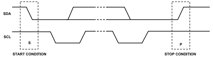
Figure 53. Start and Stop Conditions
