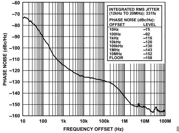
Figure 3. Absolute Phase Noise (Output Driver = HSTL), f_R = 19.44 MHz, f_{OUT} = 156.25 MHz, DPLL Loop BW = 50 Hz, f_{SYS} = 49.152 MHz Crystal
