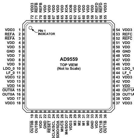
Figure 2. Pin Configuration
