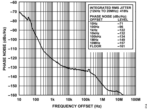
Figure 15. Absolute Phase Noise (Output Driver = 1.8V CMOS), f_R = 2\text{ kHz} , f_{OUT} = 70.656\text{ MHz} , DPLL Loop BW = 10 Hz, f_{SYS} = 19.2\text{ MHz} TCXO
