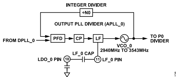
Figure 40. APLL_0 Block Diagram
