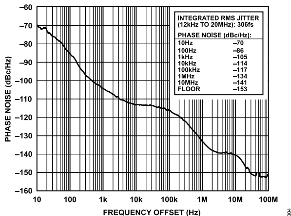
Figure 5. Absolute Phase Noise (Output Driver = HSTL), f_R = 19.44 MHz, f_{OUT} = 644.53125 MHz, DPLL Loop BW = 50 Hz, f_{SYS} = 49.152 MHz Crystal
