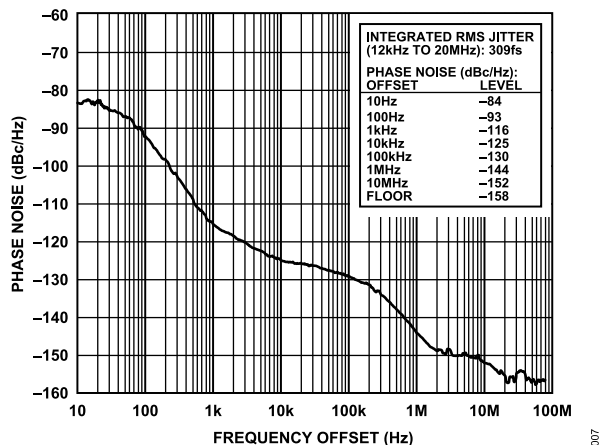
Figure 8. Absolute Phase Noise (Output Driver = 3.3V CMOS), f_R = 19.44 MHz, f_{OUT} = 161.1328125 MHz, DPLL Loop BW = 100 Hz, f_{SYS} = 49.152 MHz Crystal
