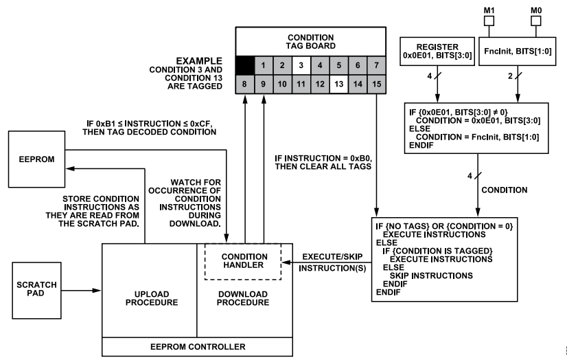
Figure 45. EEPROM Conditional Processing
