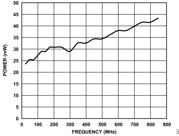
Figure 21. Power Consumption vs. Frequency, LVDS Mode on Output Driver Power Supply Only (Pin 17, Pin 21, Pin 34, and Pin 38)
