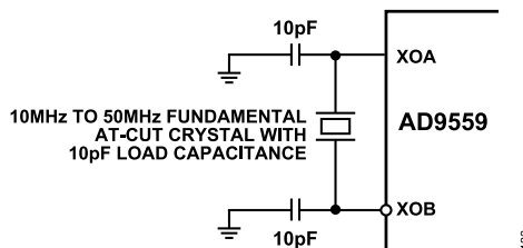
Figure 33. System Clock Input (XOA/XOB) in Crystal Mode (The recommended C_{LOAD} = 10\text{ pF} is shown. The values of 10 pF shunt capacitors shown here should equal the C_{LOAD} of the crystal.)
