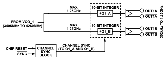
Figure 43. Clock Distribution Block Diagram from VCO_1
