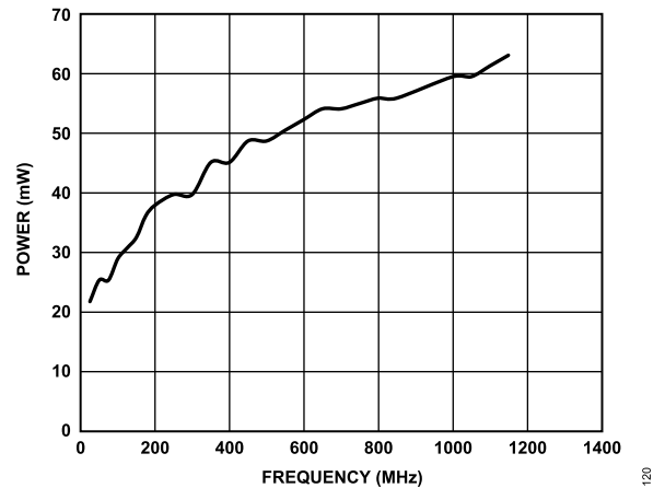
Figure 20. Power Consumption vs. Frequency, HSTL Mode on Output Driver Power Supply Only (Pin 17, Pin 21, Pin 34, and Pin 38)
