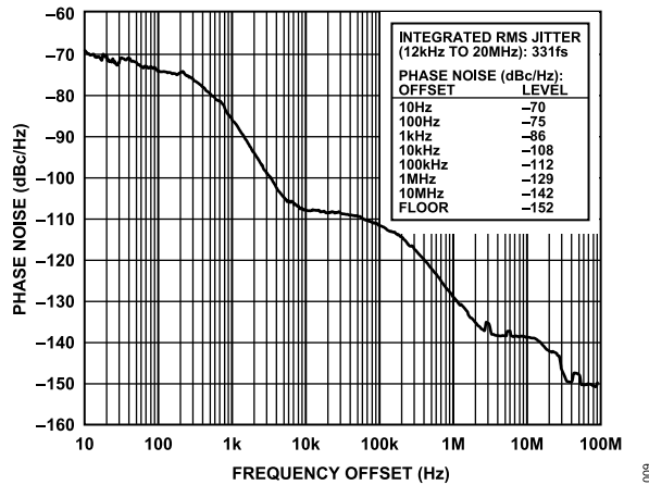
Figure 10. Absolute Phase Noise (Output Driver = HSTL), f_R = 25 MHz, f_{OUT} = 1 GHz, DPLL Loop BW = 500 Hz, f_{SYS} = 49.152 MHz Crystal
