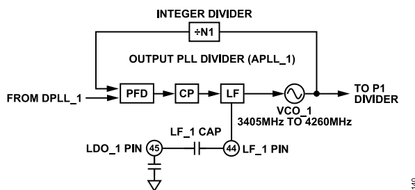
Figure 41. APLL_1 Block Diagram
