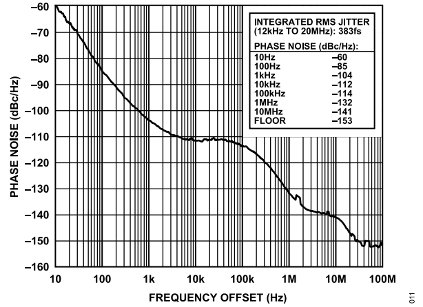
Figure 12. Absolute Phase Noise (Output Driver = HSTL), f_R = 19.44 MHz, f_{OUT} = 693.482991 MHz, DPLL Loop BW = 10 Hz, f_{SYS} = 19.2 MHz TCXO
