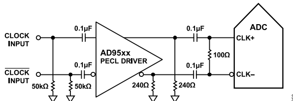
Figure 54. Differential PECL Sample Clock (Up to 625 MHz)
