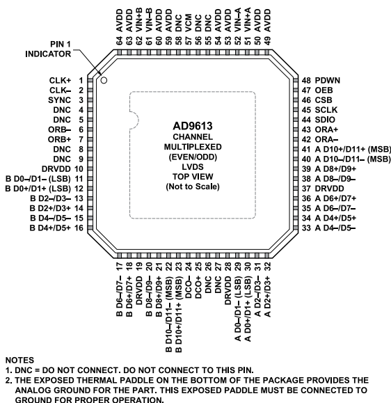
Figure 5. Pin Configuration (Top View) for the LFCSP Channel Multiplexed (Even/Odd) LVDS Mode
