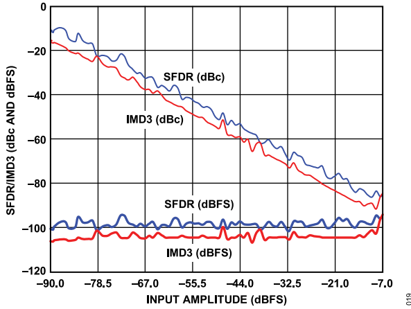
Figure 12. AD9613-170 Two-Tone SFDR/IMD3 vs. Input Amplitude ( A_{IN} ) with f_{IN1} = 184.12 , f_{IN2} = 187.12 MHz, f_s = 170 MSPS
