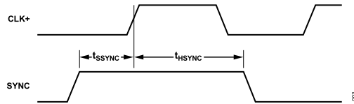
Figure 3. SYNC Timing Inputs
