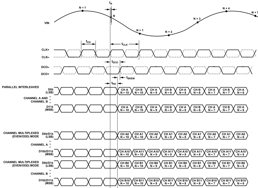
Figure 2. Interleaved LVDS Mode Data Output Timing
