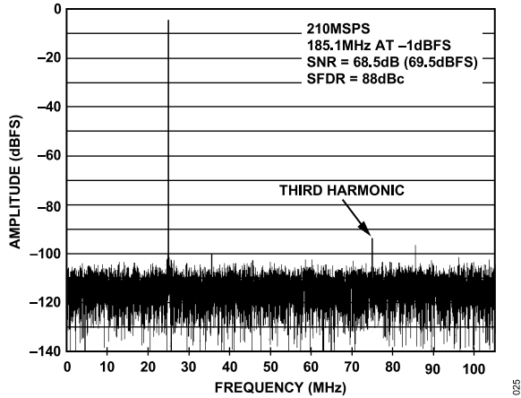
Figure 18. AD9613-210 Single-Tone FFT with f_{IN} = 185.1 MHz
