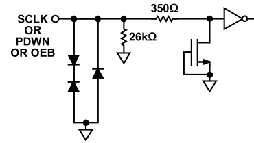
Figure 43. Equivalent SCLK, PDWN, or OEB Input Circuit
