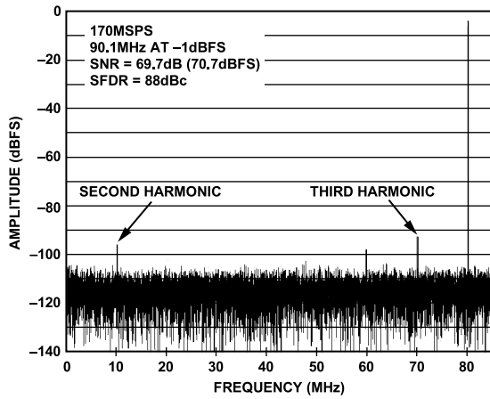
Figure 6. AD9613-170 Single-Tone FFT with f_{IN} = 90.1 MHz
