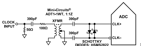
Figure 52. Transformer Coupled Differential Clock (Up to 200 MHz)
