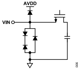
Figure 39. Equivalent Analog Input Circuit
