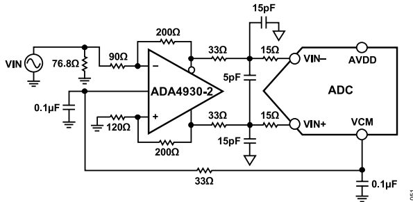
Figure 47. Differential Input Configuration Using the ADA4930-2
