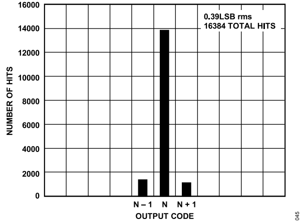
Figure 38. AD9613-250 Grounded Input Histogram
