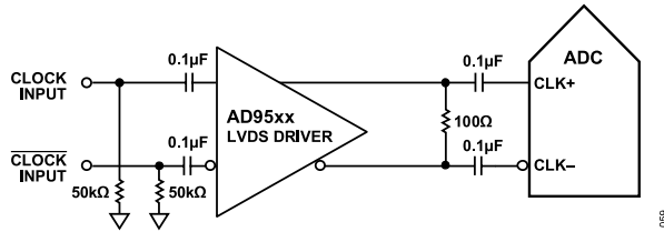
Figure 55. Differential LVDS Sample Clock (Up to 625 MHz)
