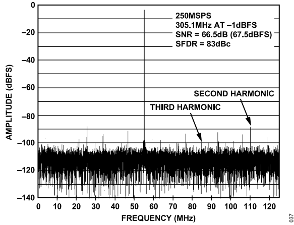
Figure 30. AD9613-250 Single-Tone FFT with f_{IN} = 305.1 MHz
