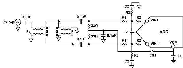
Figure 49. Differential Double Balun Input Configuration
