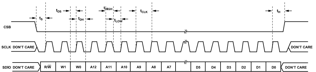
Figure 58. Serial Port Interface Timing Diagram
