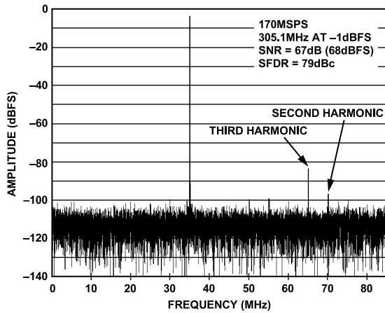
Figure 8. AD9613-170 Single-Tone FFT with f_{IN} = 305.1 MHz
