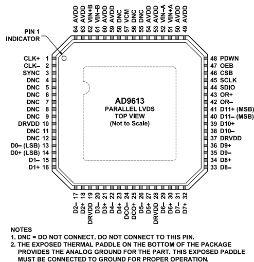
Figure 4. Pin Configuration (Top View) for the LFCSP Interleaved Parallel LVDS Mode
