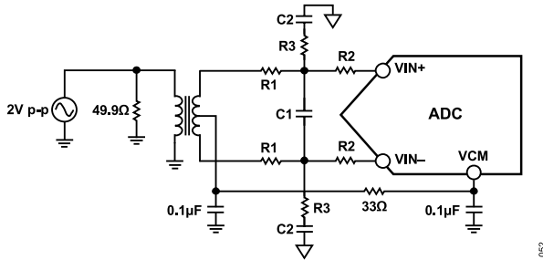
Figure 48. Differential Transformer-Coupled Configuration
