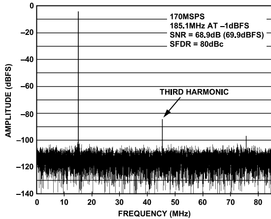
Figure 7. AD9613-170 Single-Tone FFT with f_{IN} = 185.1 MHz
