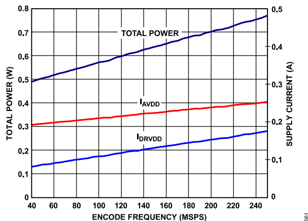
Figure 57. AD9613-250 Power and Current vs. Sample Rate
