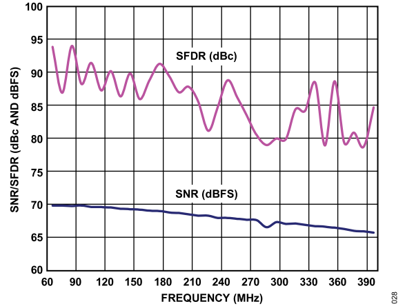
Figure 21. AD9613-210 Single-Tone SNR/SFDR vs. Input Frequency ( f_{IN} )
