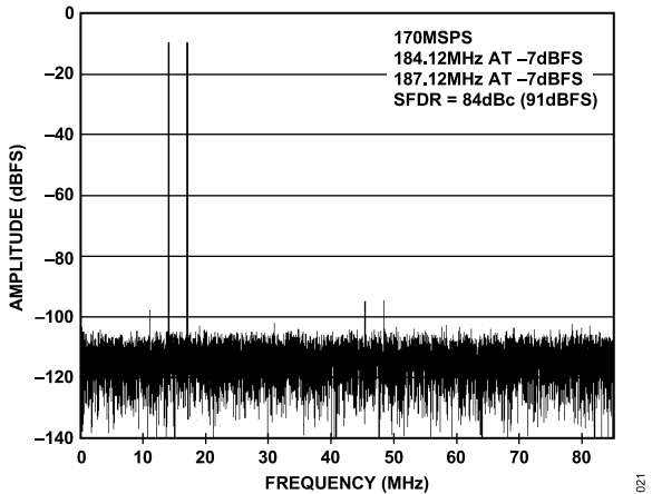
Figure 14. AD9613-170 Two-Tone FFT with f_{IN1} = 184.12 , f_{IN2} = 187.12 MHz, f_s = 170 MSPS
