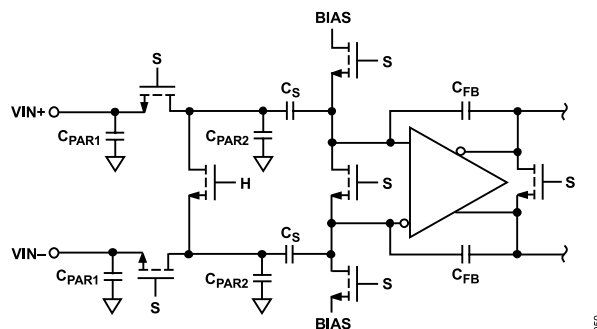
Figure 46. Switched-Capacitor Input
