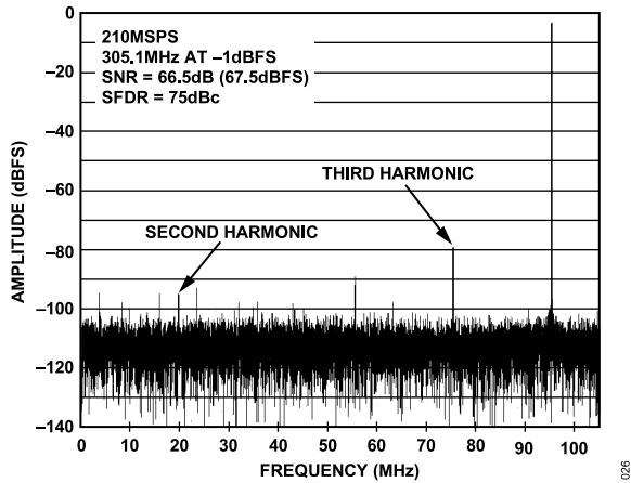
Figure 19. AD9613-210 Single-Tone FFT with f_{IN} = 305.1 MHz
