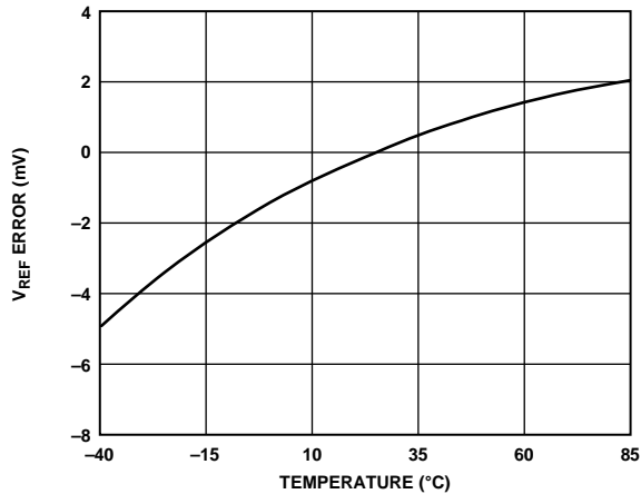
Figure 54. Typical VREF Drift
