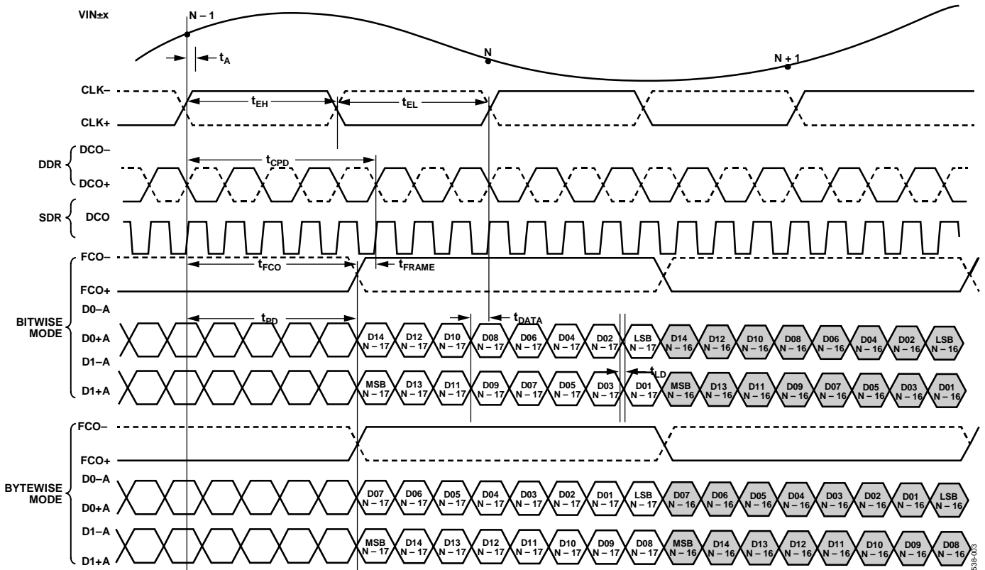
Figure 3. 16-Bit DDR/SDR, Two-Lane, 2x Frame Mode
