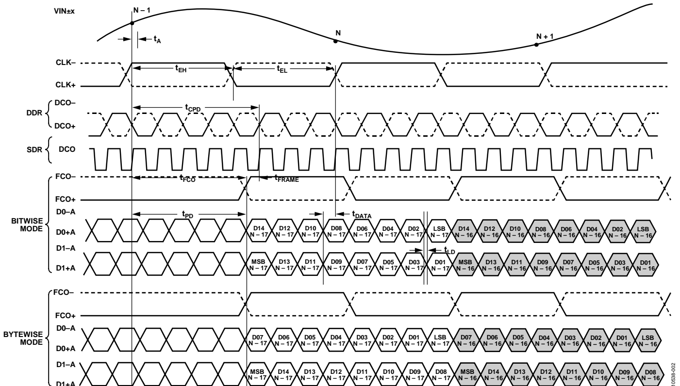
Figure 2. 16-Bit DDR/SDR, Two-Lane, 1x Frame Mode (Default)
