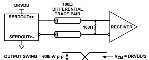
Figure 48. DC-Coupled Digital Output Termination Example
