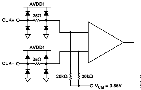
Figure 105. Clock Inputs
