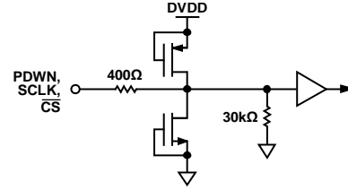
Figure 38. Equivalent PDWN, SCLK, or \overline{CS} Input Circuit
