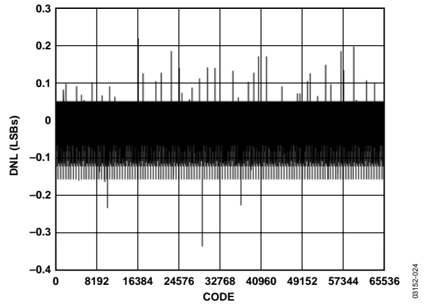
Figure 24. Typical DNL
