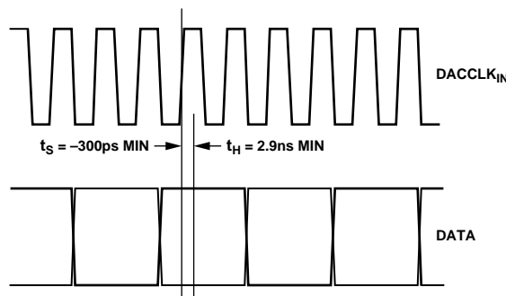
Figure 53. External Sync Mode with 2x Interpolation
