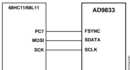
Figure 29. 68HC11/68L11 to AD9833 Interface
