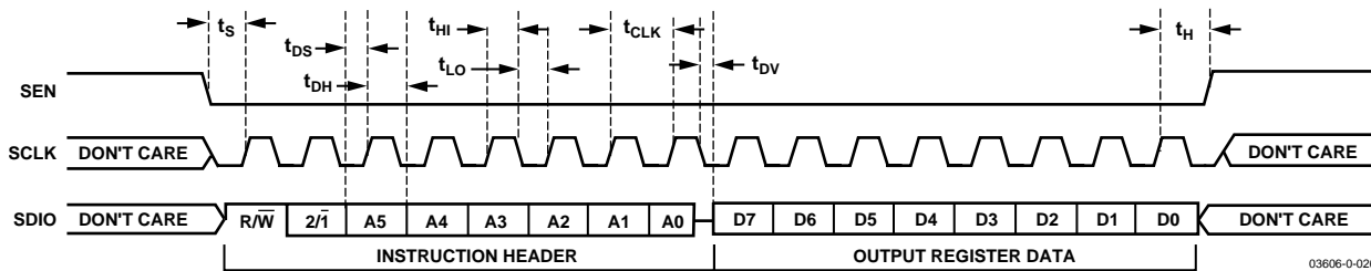
Figure 82. 1-Byte Serial Register Readback in MSB First Mode, SDIO BiDir Bit Set Logic High (Default, 3-Wire Mode)
