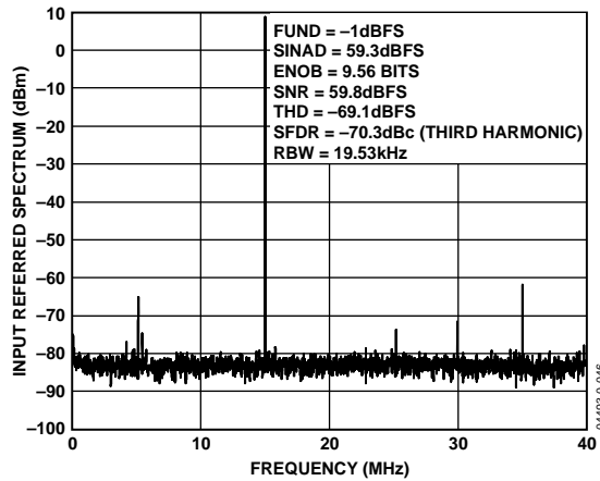
Figure 9. Spectral Plot with 4k FFT of Input Sinusoid with RxPGA = 0 dB and P_{IN} = 9 dBm
