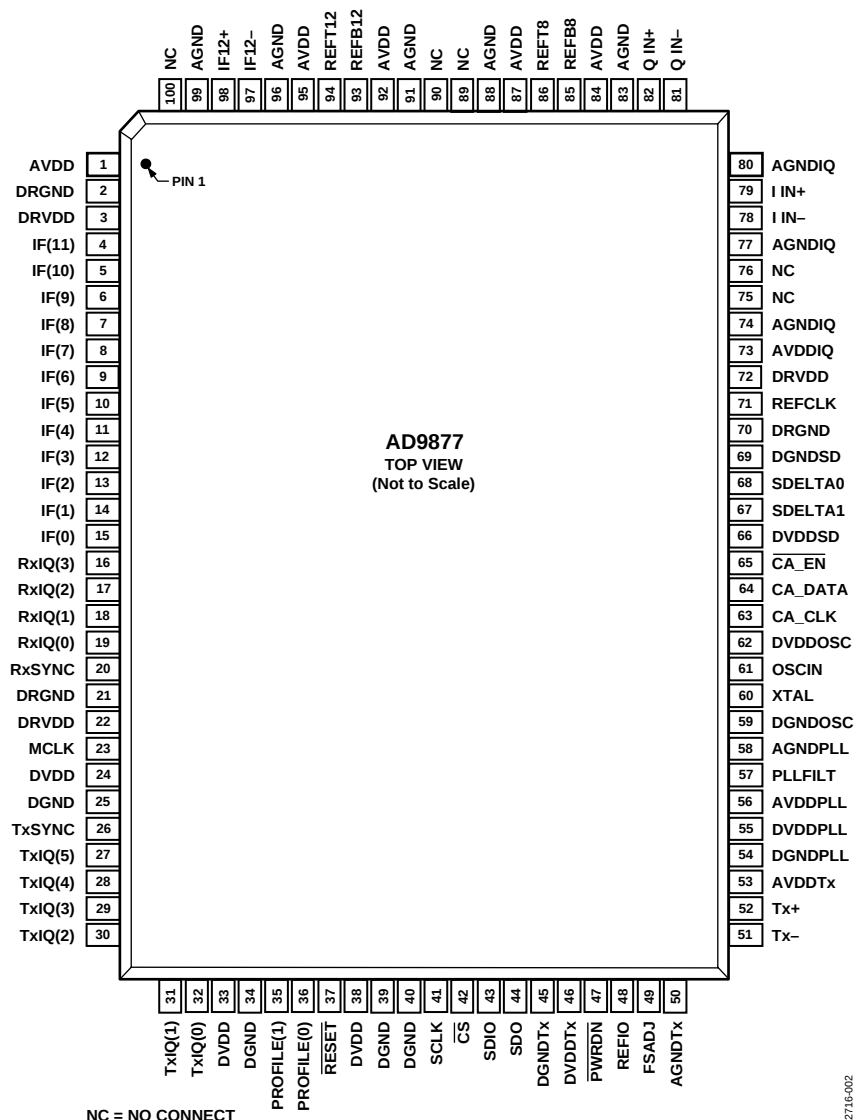
Figure 2. Pin Configuration
