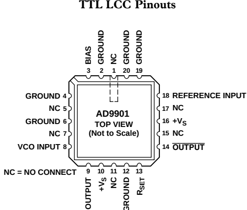
TTL LCC Pinouts
