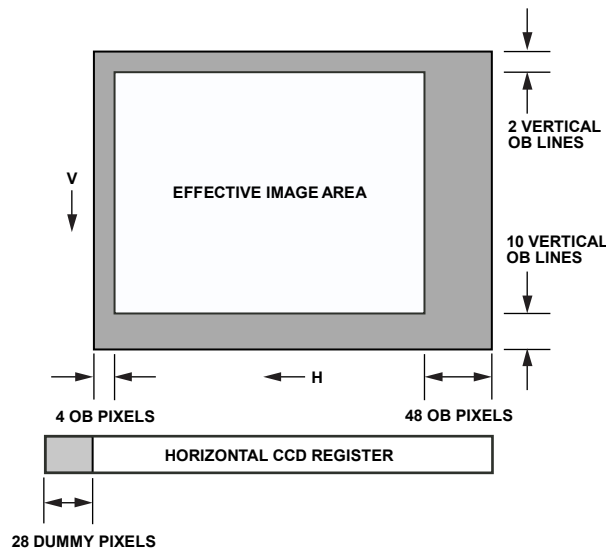
Figure 32. Example CCD Configuration
