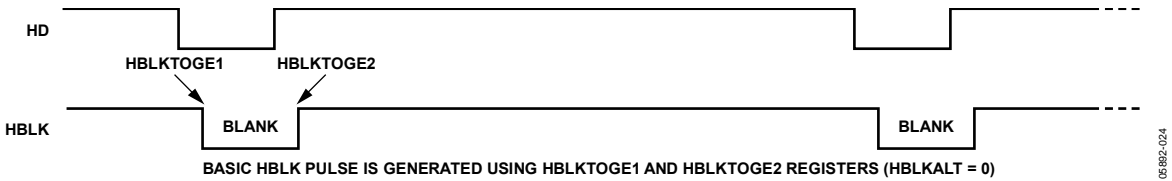
Figure 25. Typical Horizontal Blanking Pulse Placement (HBLKMODE = 0)
