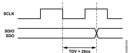
Figure 28. Serial Port I/O Data Valid Time (TDV) During Readback
