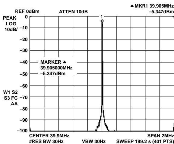
Figure 11. F_{OUT} = 39.9 MHz, F_{CLK} = 400 MSPS, NBSFDR, \pm 1 MHz
