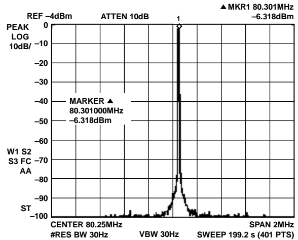
Figure 12. F_{OUT} = 80.3 MHz, F_{CLK} = 400 MSPS, NBSFDR, \pm 1 MHz
