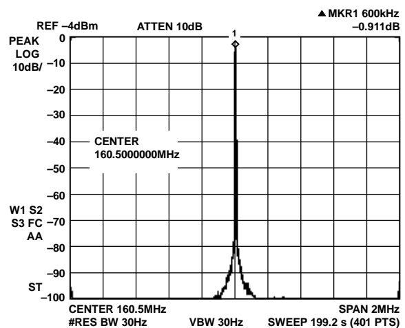
Figure 14. F_{OUT} = 160 MHz, F_{CLK} = 400 MSPS, NBSFDR, \pm 1 MHz
