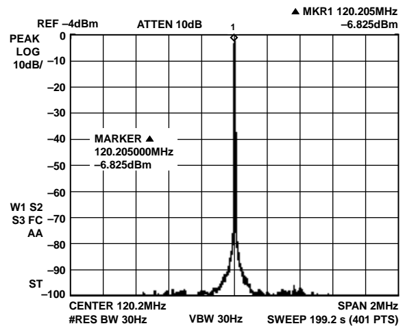
Figure 13. F_{OUT} = 120.2 MHz, F_{CLK} = 400 MSPS, NBSFDR, \pm 1 MHz
