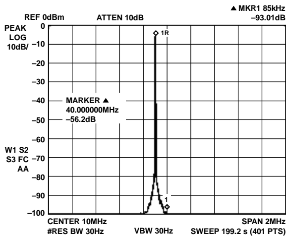
Figure 10. F_{OUT} = 10 MHz, F_{CLK} = 400 MSPS, NBSFDR, \pm 1 MHz
