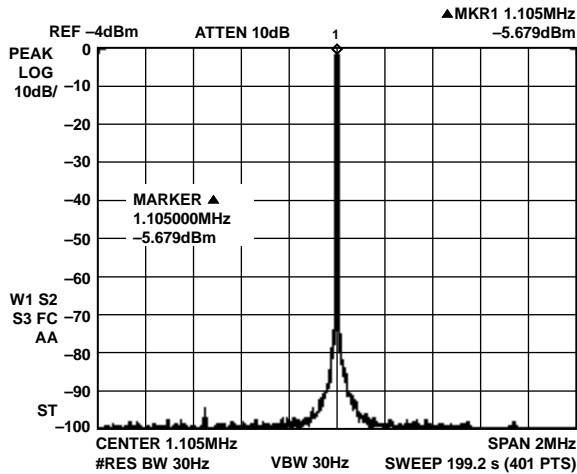
Figure 9. F_{OUT} = 1.1 MHz, F_{CLK} = 400 MSPS, NBSFDR, \pm 1 MHz
