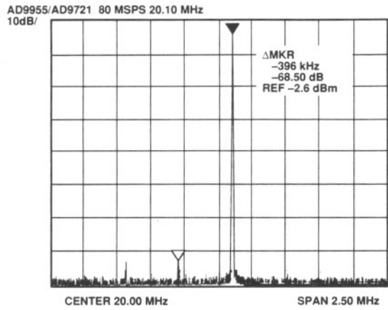
Figure 17. AD9955/AD9721 Output Spectrum
