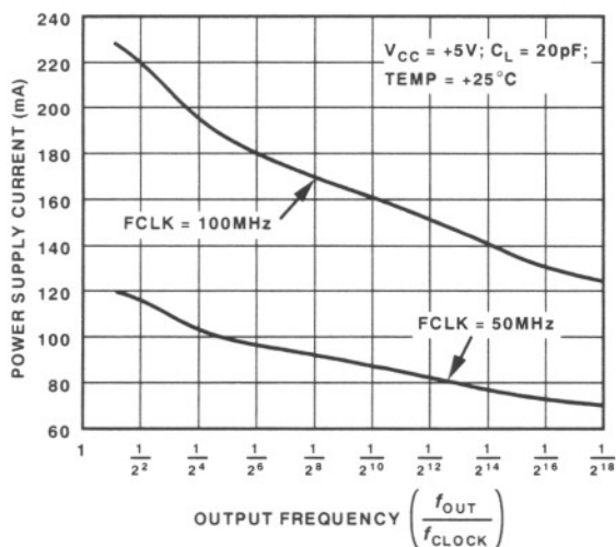
Figure 3. Power Supply Current vs. Output Frequency
