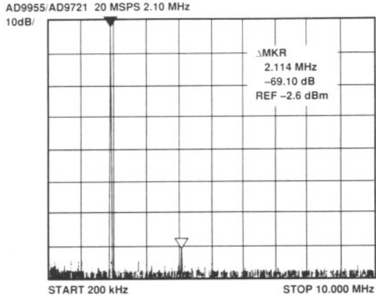
Figure 10. AD9955/AD9721 Output Spectrum
