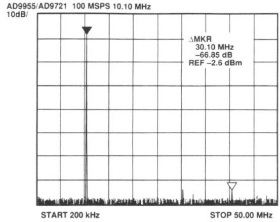
Figure 19. AD9955/AD9721 Output Spectrum
