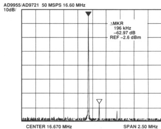
Figure 15. AD9955/AD97212 Output Spectrum
