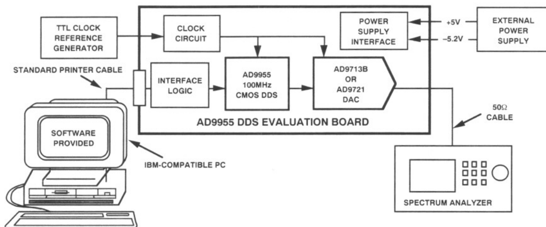
Figure 9. AD9955 DDS Evaluation Board Setup
