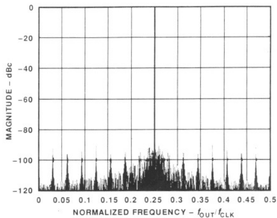
Figure 8. AD9955 Output Spectrum
