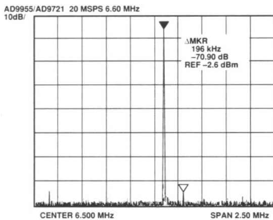
Figure 12. AD9955/AD9721 Output Spectrum
