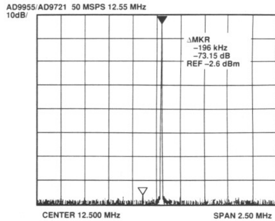
Figure 14. AD9955/AD9721 Output Spectrum
