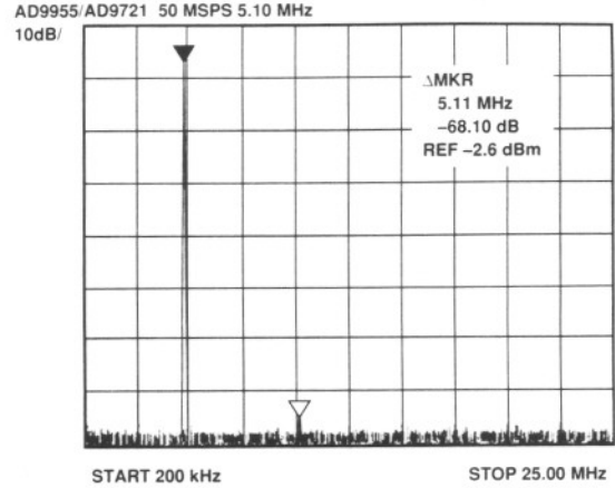
Figure 13. AD9955/AD9721 Output Spectrum
