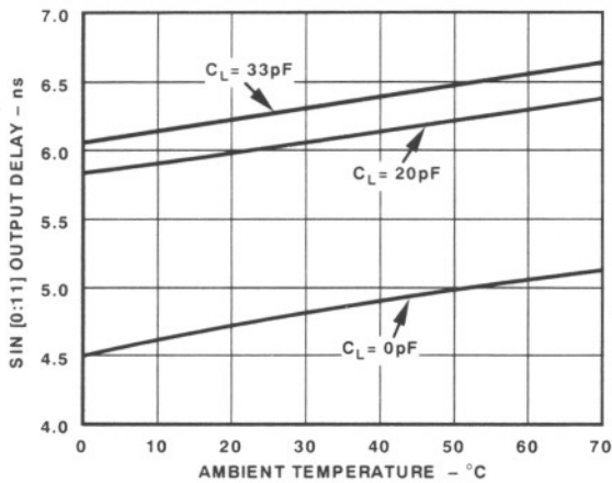
Figure 6. Output Delay vs. Ambient Temperature
