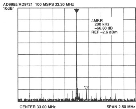
Figure 21. AD9955/AD9721 Output Spectrum
