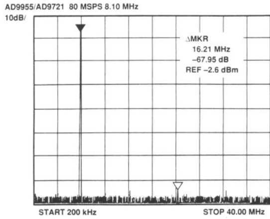
Figure 16. AD9955/AD9721 Output Spectrum
