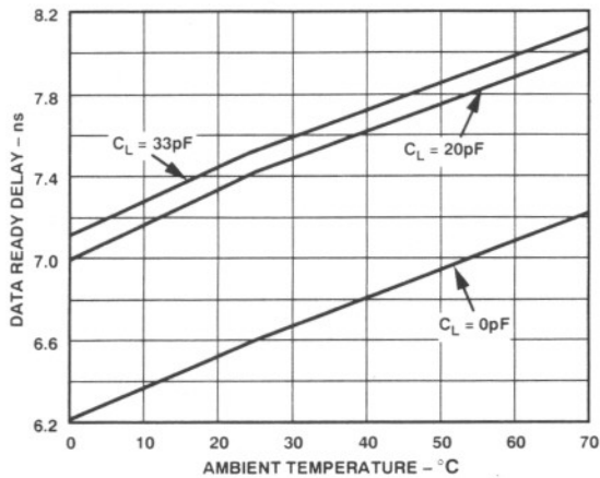
Figure 5. Data Ready Delay vs. Ambient Temperature
