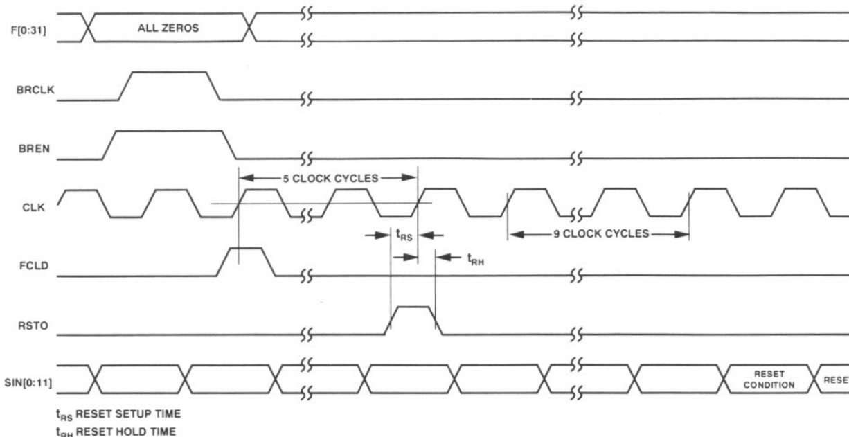
Figure 2. Reset Timing
