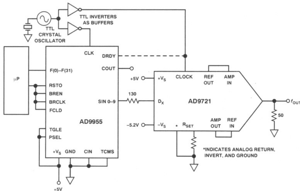
Figure 7. AD9955/AD9721 DDS Synthesizer
