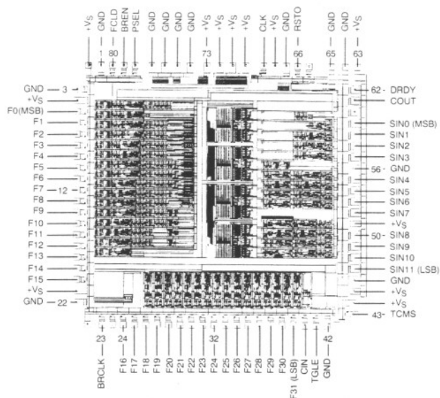
AD9955 Chip Layout
