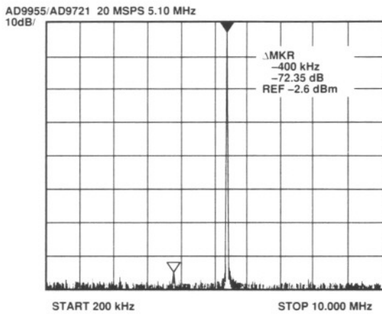
Figure 11. AD9955/AD9721 Output Spectrum
