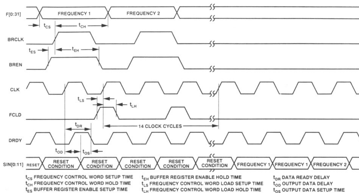
Figure 4. Parallel Mode Timing
