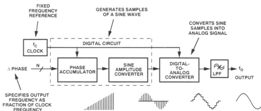
Figure 1. Block Diagram of DDS Generator
