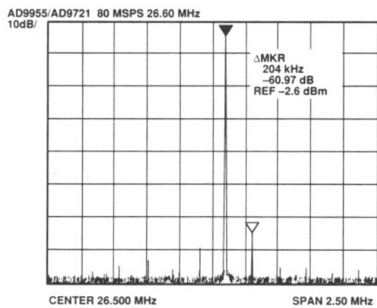
Figure 18. AD9955/AD9721 Output Spectrum
