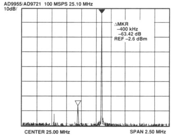
Figure 20. AD9955/AD9721 Output Spectrum
